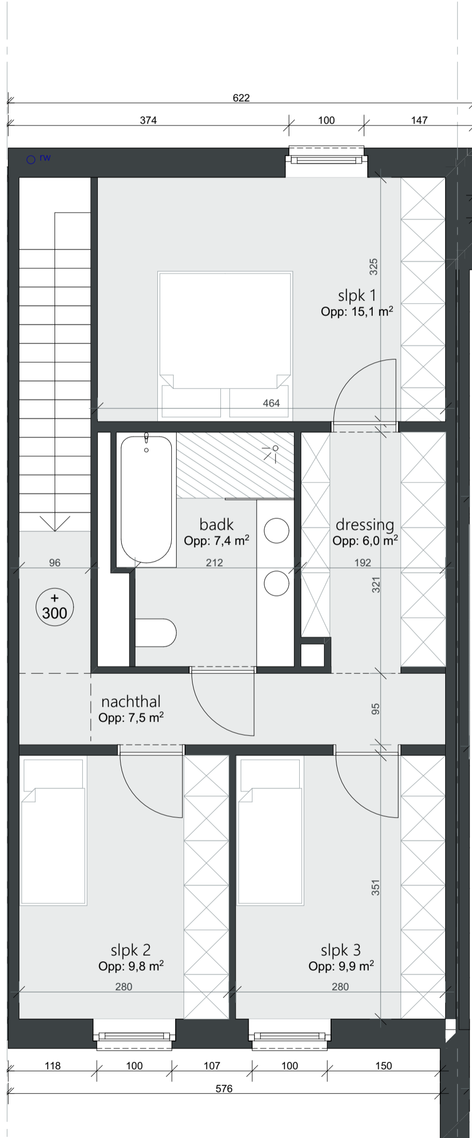
Grond plan: niv +1
